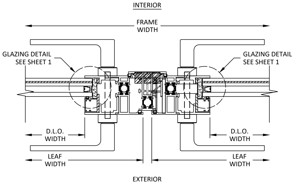
G 6 HORIZONTAL SECTION MEETING STILE - LOCK
