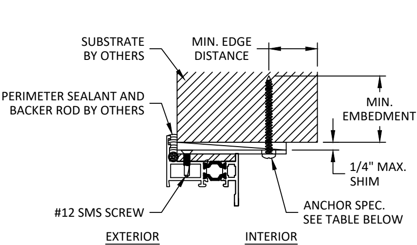
I 7 INSTALLATION DETAILS HEAD SHOWN, JAMB SIMILAR ANCHOR THROUGH STRAP ONLY
