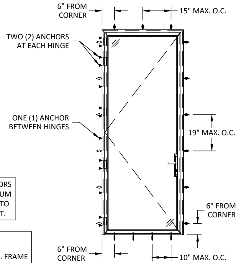
ANCHOR LAYOUT SINGLE DOOR, THRU. STRAP & FRAME
