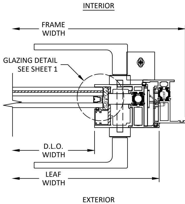
H 6 HORIZONTAL SECTION LOCK JAMB - LOCK
