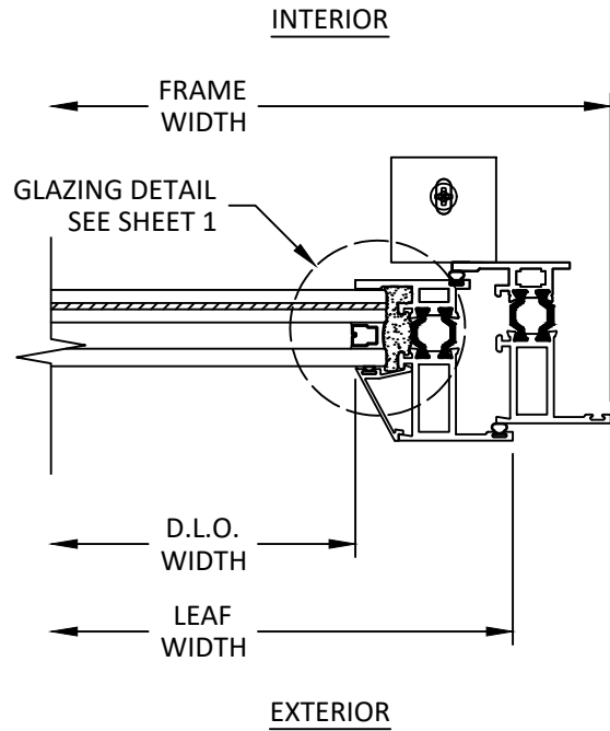
F 6 HORIZONTAL SECTION LOCK JAMB
