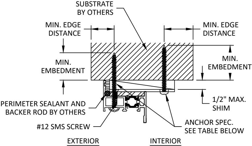
J 7 INSTALLATION DETAILS HEAD SHOWN, JAMB SIMILAR ANCHOR THROUGH STRAP AND FRAME
