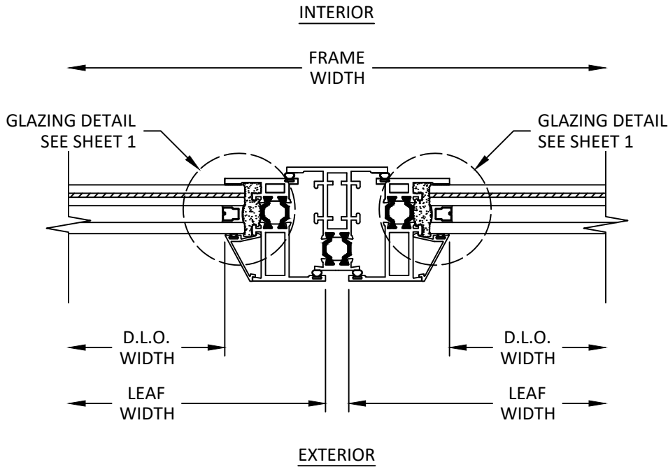
E 6 HORIZONTAL SECTION MEETING STILE
