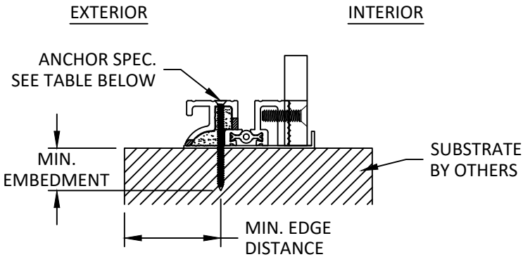
K 7 INSTALLATION DETAILS SILL SHOWN
