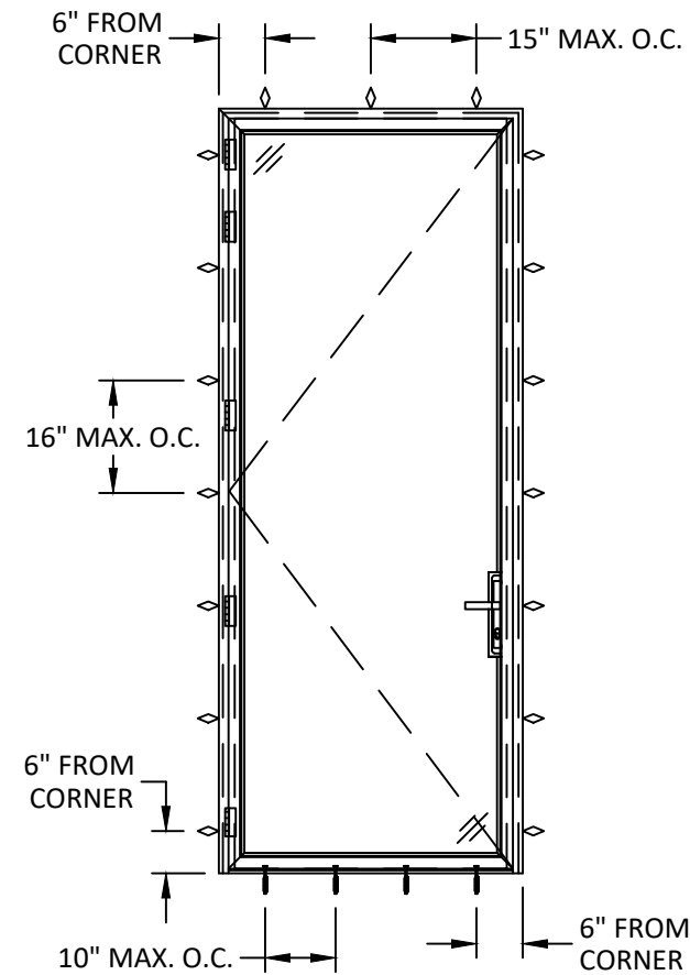
ANCHOR LAYOUT SINGLE DOOR, THRU. STRAP ONLY
